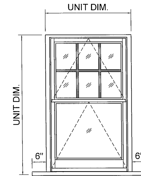
EXTERIOR ELEVATION OF SERIES 4000 DOUBLE HUNG FOLD-UP IN WINDOW UNIT WITH SILL
